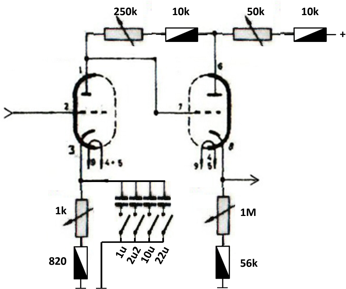
William Jehle 12ax7 Cathode Follower / \mu Multiplier 12 NOV 2024
