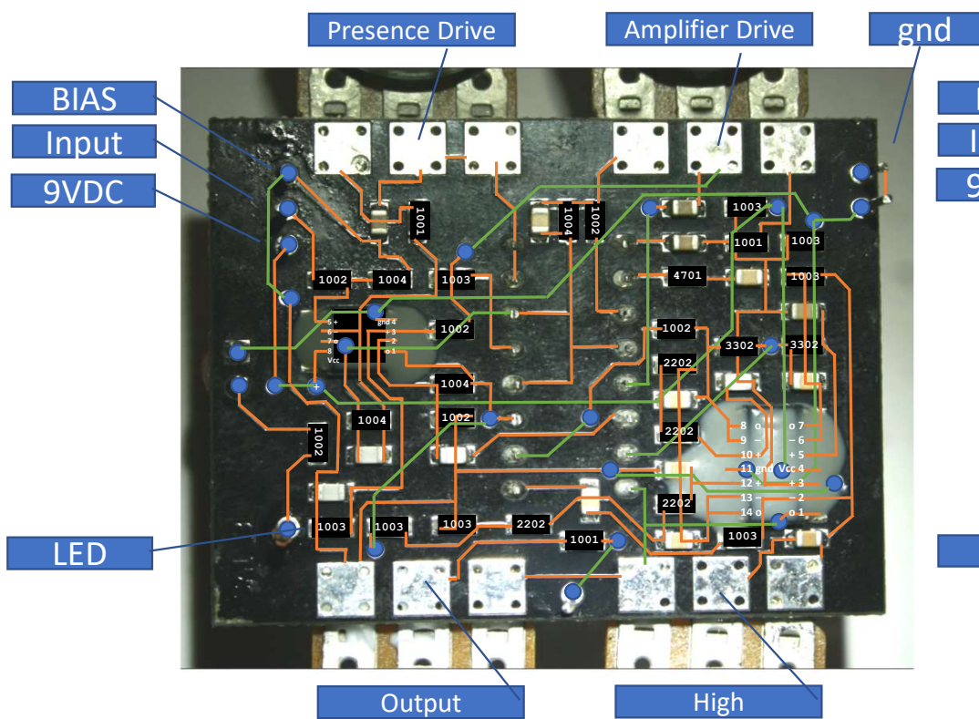
Comparison of replacement board to original (from original Japanese board?)
