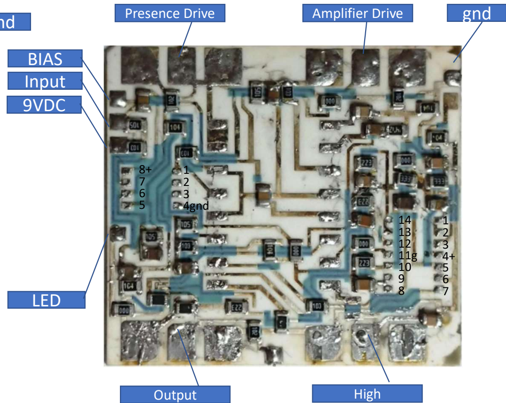
Mirror copy of original board to match new one Resistor values mirrored back for readability Opamps are now backwards (sorry)
