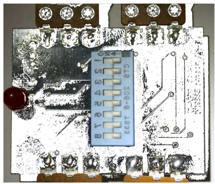
Photo of deconstructed replacement board. Attempted mirror image of reverse (top) side for traces and mapping vias.
